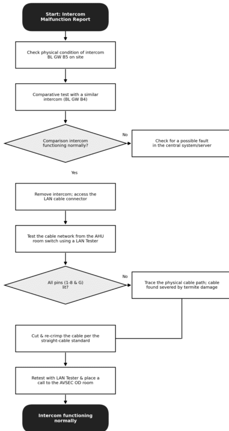
Figure 1 Flowchart of the Access Control Intercom Malfunction Diagnosis and Handling Process (Source: Processed by the Authors, 2025)
