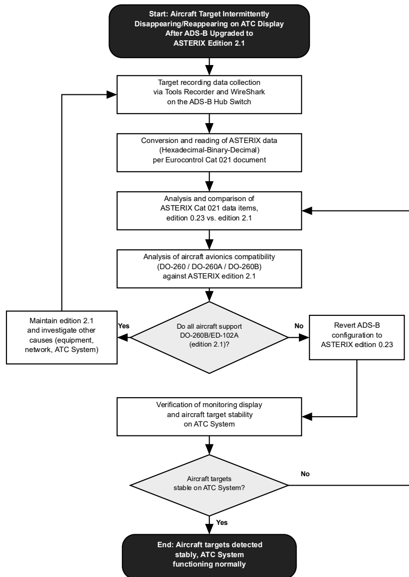
Figure 1 Flowchart of the ASTERIX ADS-B Edition 0.23 and Edition 2.1 Data Analysis at Perum LPPNPI AirNav Denpasar Branch (Source: Processed by the Authors, 2026)
