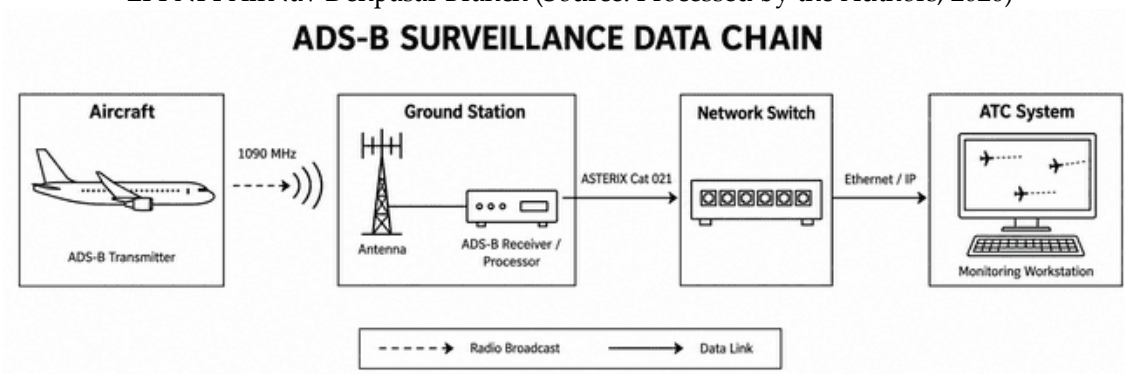
Figure 2 Conceptual Illustration of ASTERIX Data Exchange Between the Aircraft, the ADS-B Ground Station, and the ATC System (Source: Authors' illustration, based on Eurocontrol, 2011)
