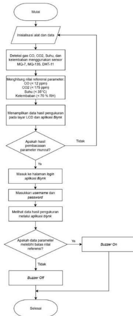
Gambar 2. Flowchart
