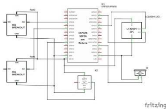
Gambar 4. Wiring Diagram
