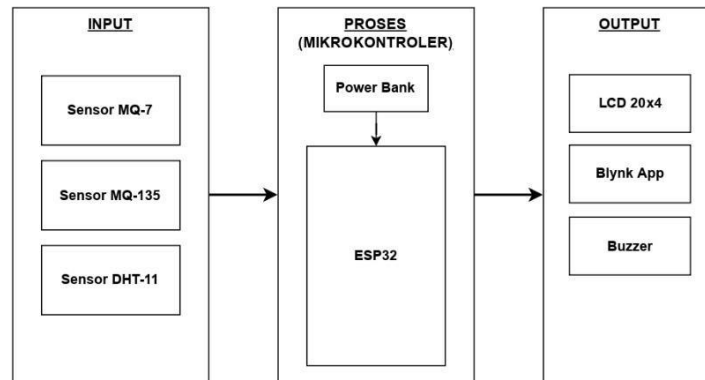
Gambar 1. Blok Diagram
