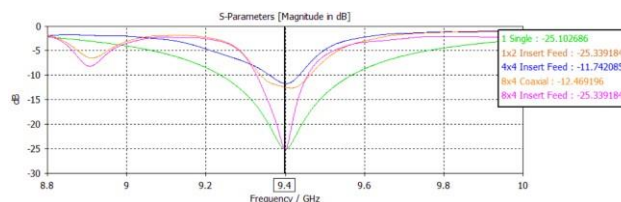
Gambar 2. Grafik Return Loss FR-4
