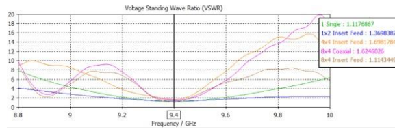
Gambar 5. Hasil Simulasi VSWR FR-4
