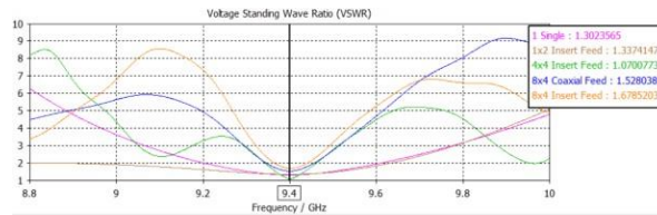
Gambar 4. Hasil Simulasi VSWR Rogers RT-5880
