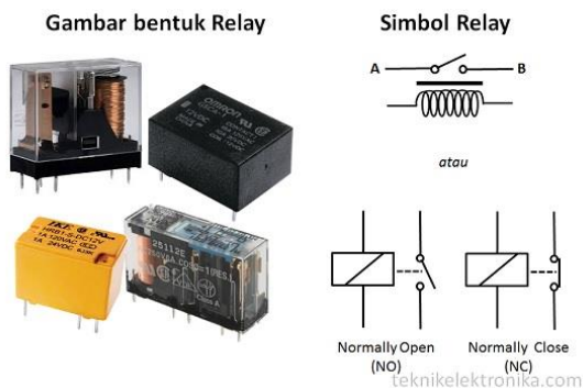
Gambar 4 Relay
