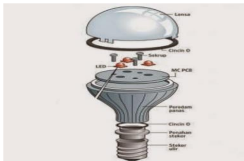
Gambar 2 Lampu LED
