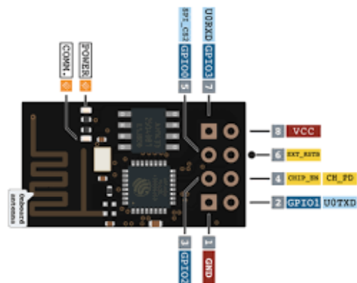
Gambar 7 ESP-01
