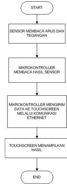
Gbr. 4. Flowchart Rangkaian Monitoring
