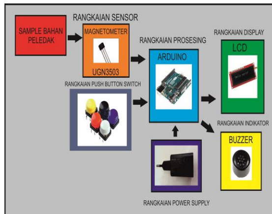
Gambar 1. Diagram blok rancangan Explosive Detector
